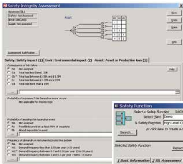
Our TRAC software offers both Risks Graph and Layer of Protection methodologies (from IEC 61511) to assess SIL requirements.
